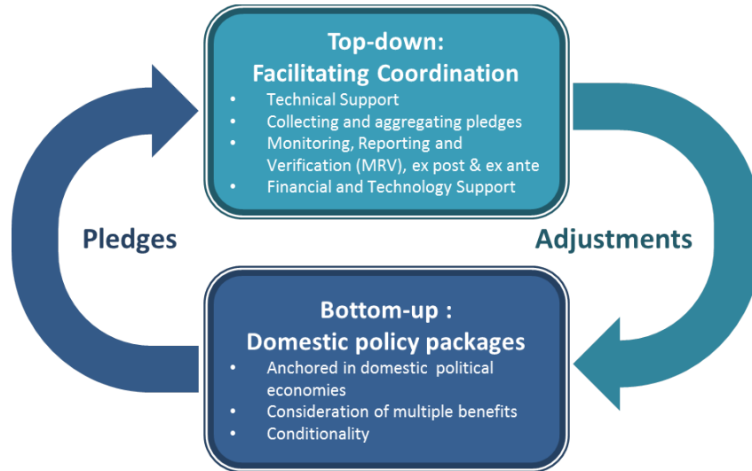
Figure 5: Structure of a dynamic hybrid climate regime (based on (Edenhofer, Flachsland, Stavins, et al. 2013))
