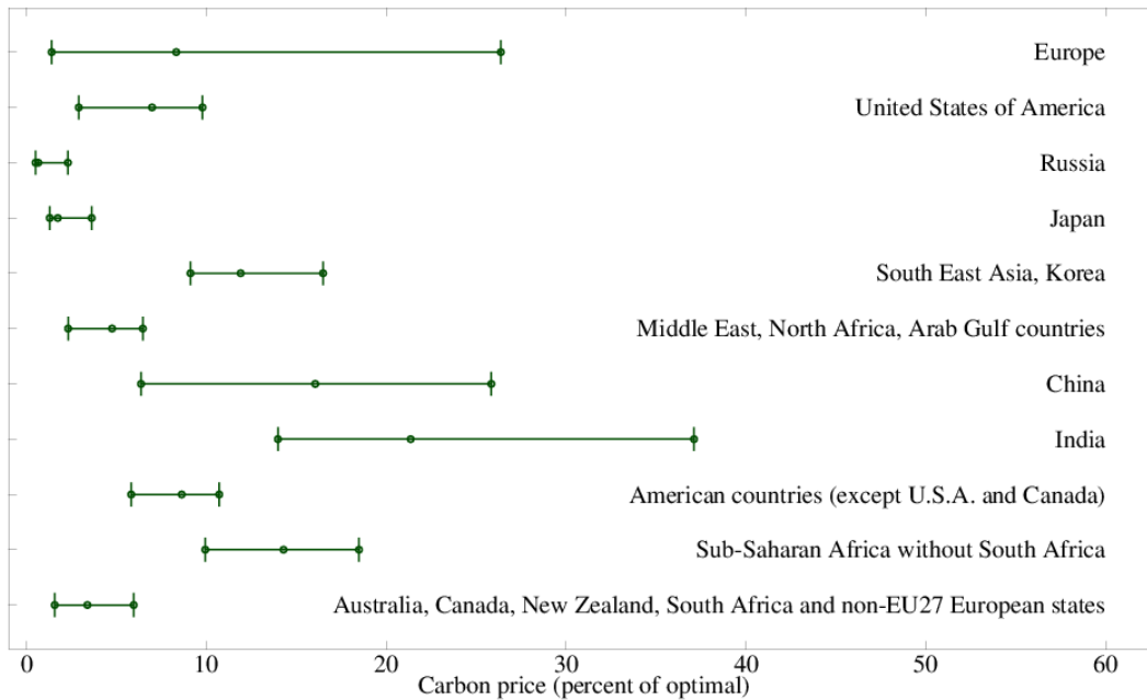
Figure 3: Unilateral carbon prices calculated with the MICA model based on different damages functions as used in the RICE (William D. Nordhaus and Joseph G. Boyer 1999) and STACO (Dellink et al. 2004) models, expressed in terms of percentage of the optimal global carbon price calculated by MICA. For details, see SI.
