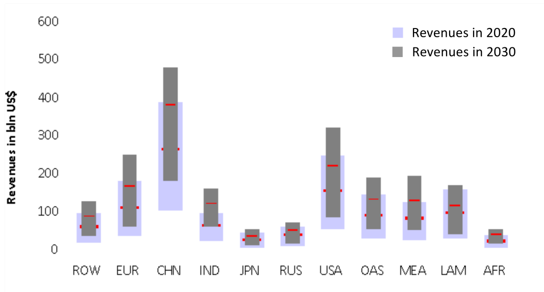
Figure 2: Amount of annual revenues in bln US$ for different regions for different tax levels in 2020 (light grey) and 2030 (dark grey). Tax levels are set to $10 (lower bound of bars), $30 (red line) and $50 (upper bound of bars) per ton of CO 2 , respectively in 2020, increasing by 5% per year. All mitigation technologies are assumed to be available. Scenarios are calculated using the ReMIND model (Leimbach et al. 2010) as described in (Luderer et al. 2013). See SI for details.
