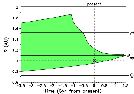
Figure 1: Evolution of the HZ for an Earth-like planet in the solar system with a total carbon amount of 10 bar and an optimum temperature of the biosphere of 50°C (Franck et al. 2000).
